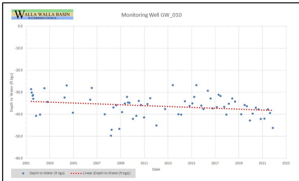
Figure 11. Manual water level measurements (blue dots) for the well GW_010 located in the WWBWC's Shallow Aquifer Monitoring Network.
