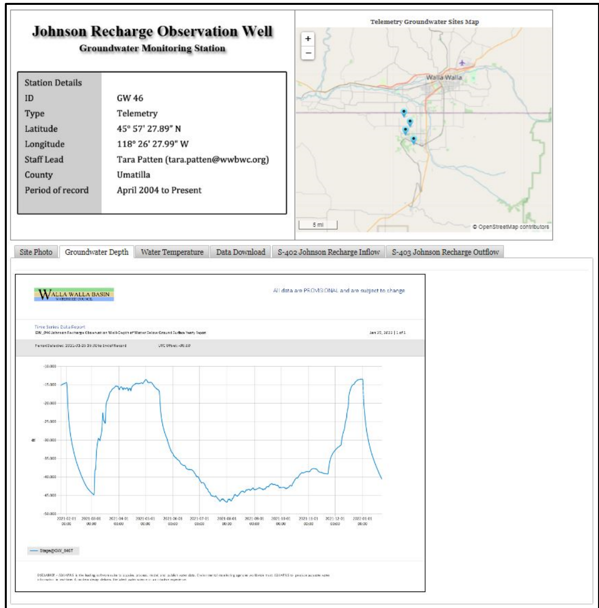
Figure 34. Example webpage for near real-time groundwater monitoring in the WWBWC's Shallow Aquifer Monitoring Network.
