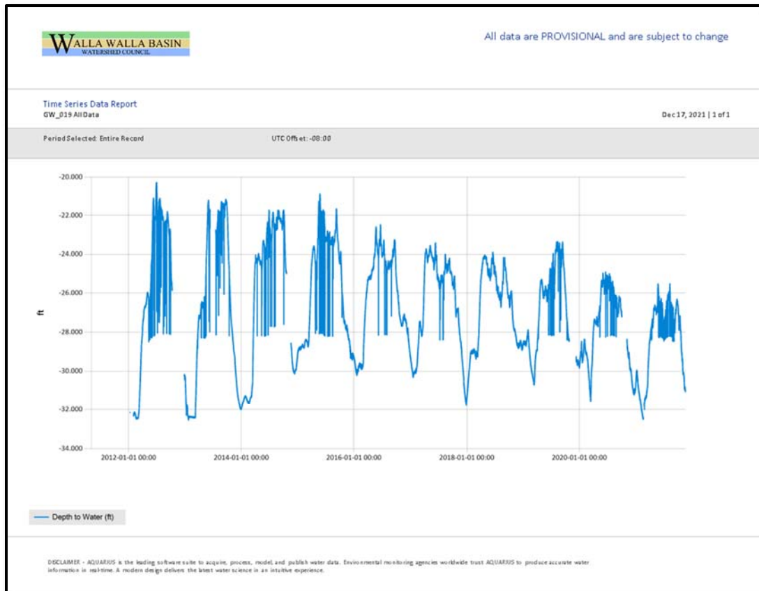
Figure 30. Pressure transducer data (blue line) in feet below ground surface for the well GW_019 located in the WWBWC's Shallow Aquifer Monitoring Network.
