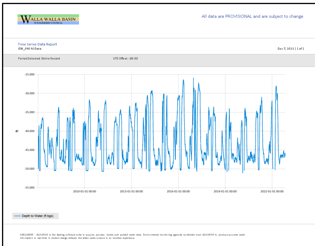
Figure 19. Pressure transducer data (blue line) in feet below ground surface for the well GW_040 located in the WWBWC's Shallow Aquifer Monitoring Network.
