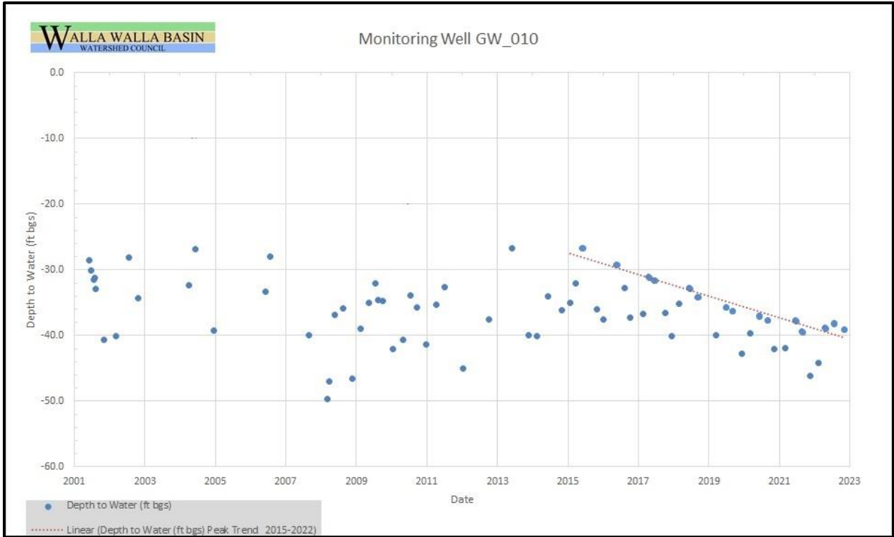
Figure 11. Manual water level measurements (blue dots) and a trend line for the high peaks from 2015-2022 (red dash line) for the well GW_010 located in the WWBWC's Shallow Aquifer Monitoring Network.
