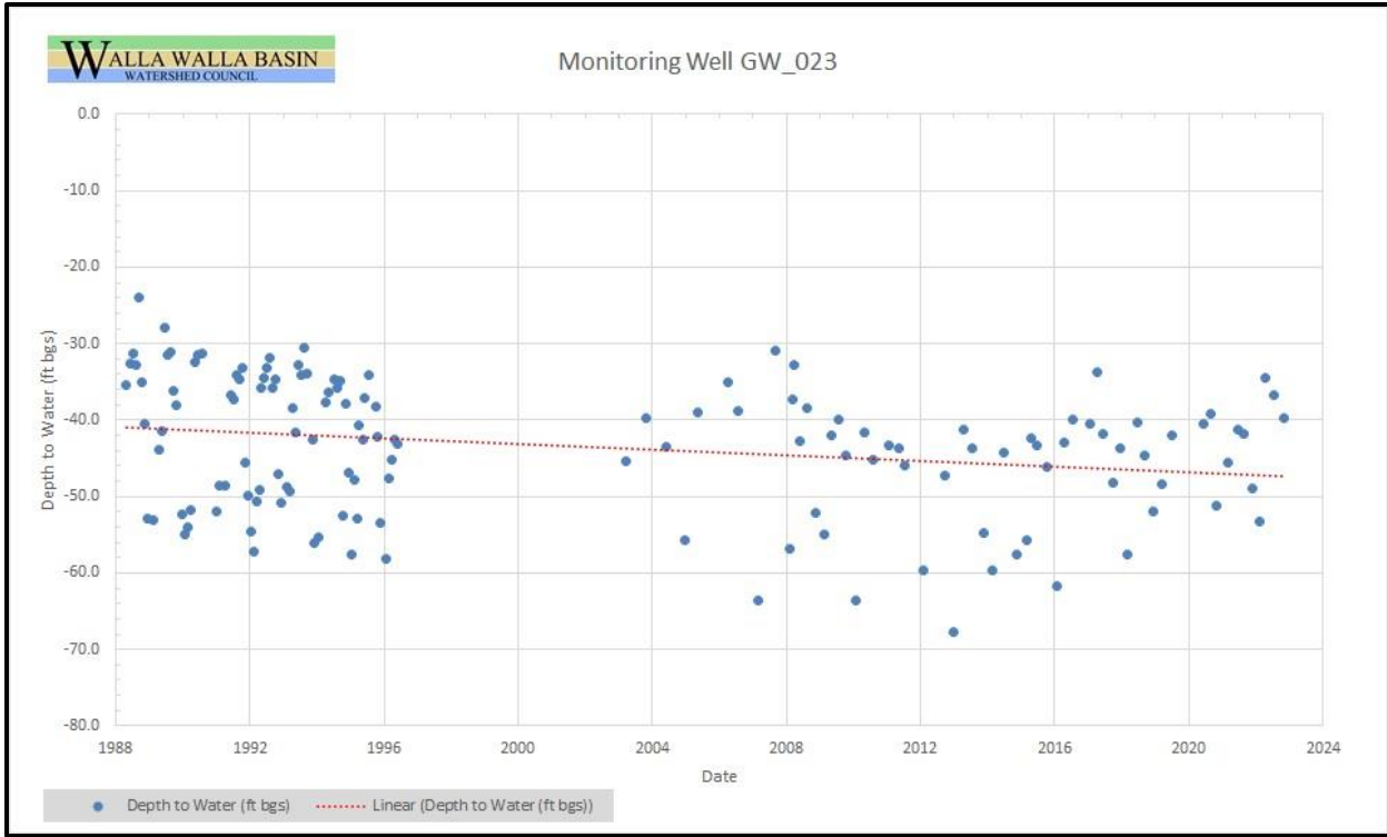
Figure 31. Manual water level measurements (blue dots) and a trend line (red dash line) for the well GW_023 located in the WWBWC's Shallow Aquifer Monitoring Network.
