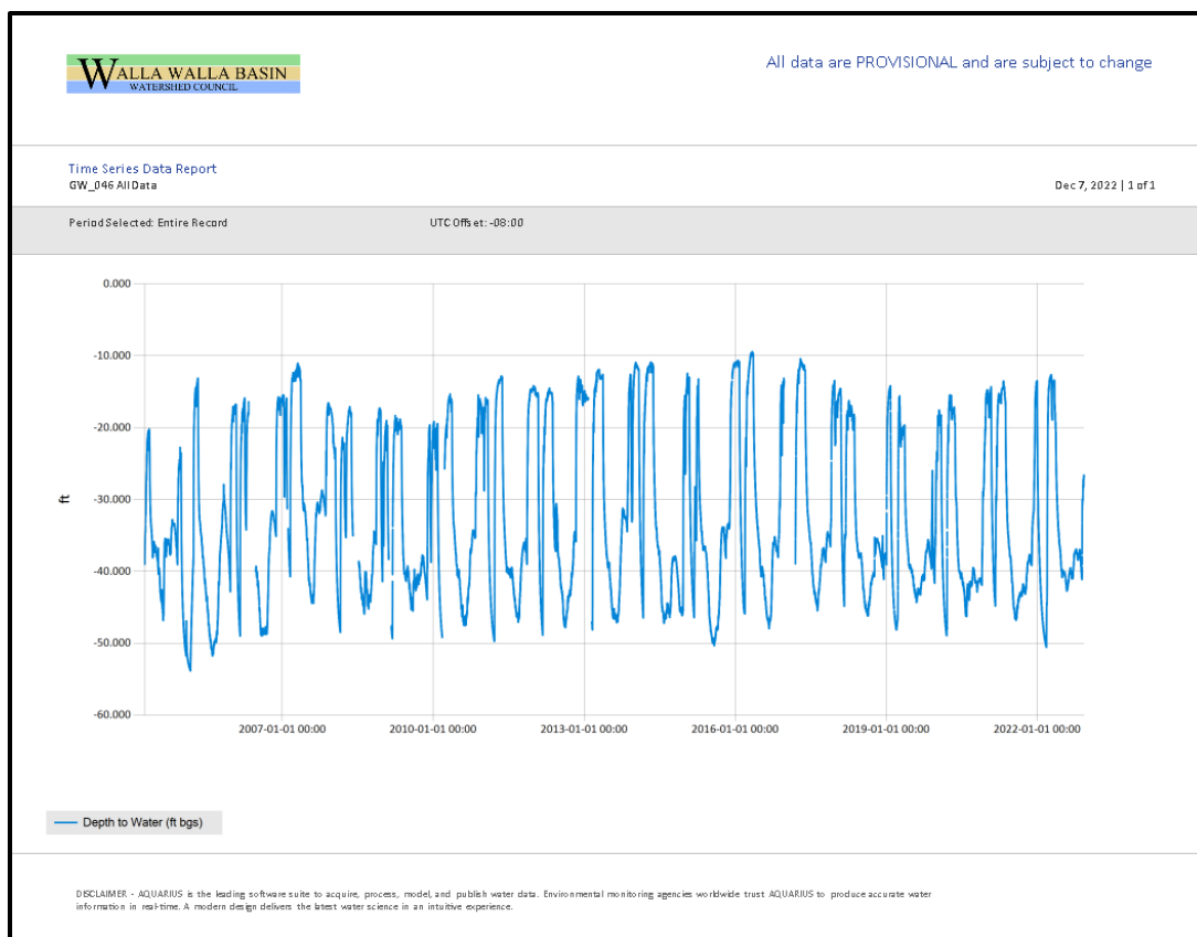
Figure 21. Pressure transducer data (blue line) in feet below ground surface for the well GW_046 located in the WWBWC's Shallow Aquifer Monitoring Network.
