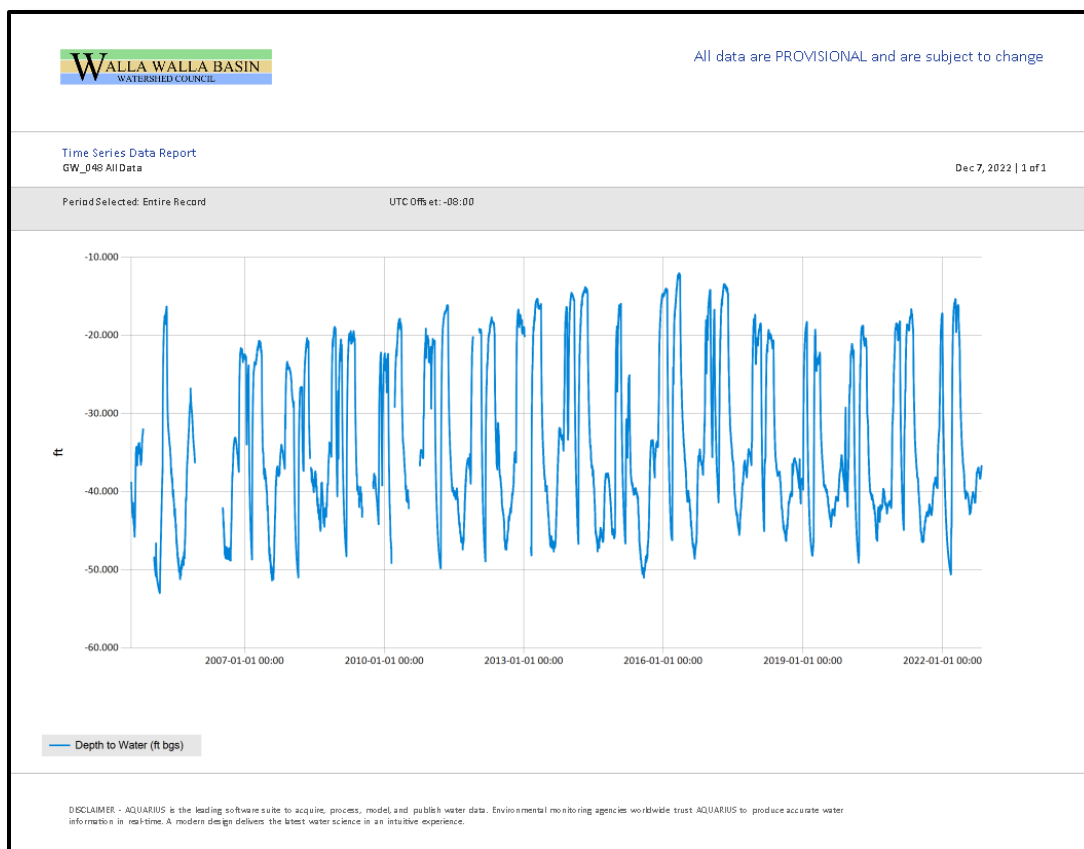
Figure 23. Pressure transducer data (blue line) in feet below ground surface for the well GW_048 located in the WWBWC's Shallow Aquifer Monitoring Network.
