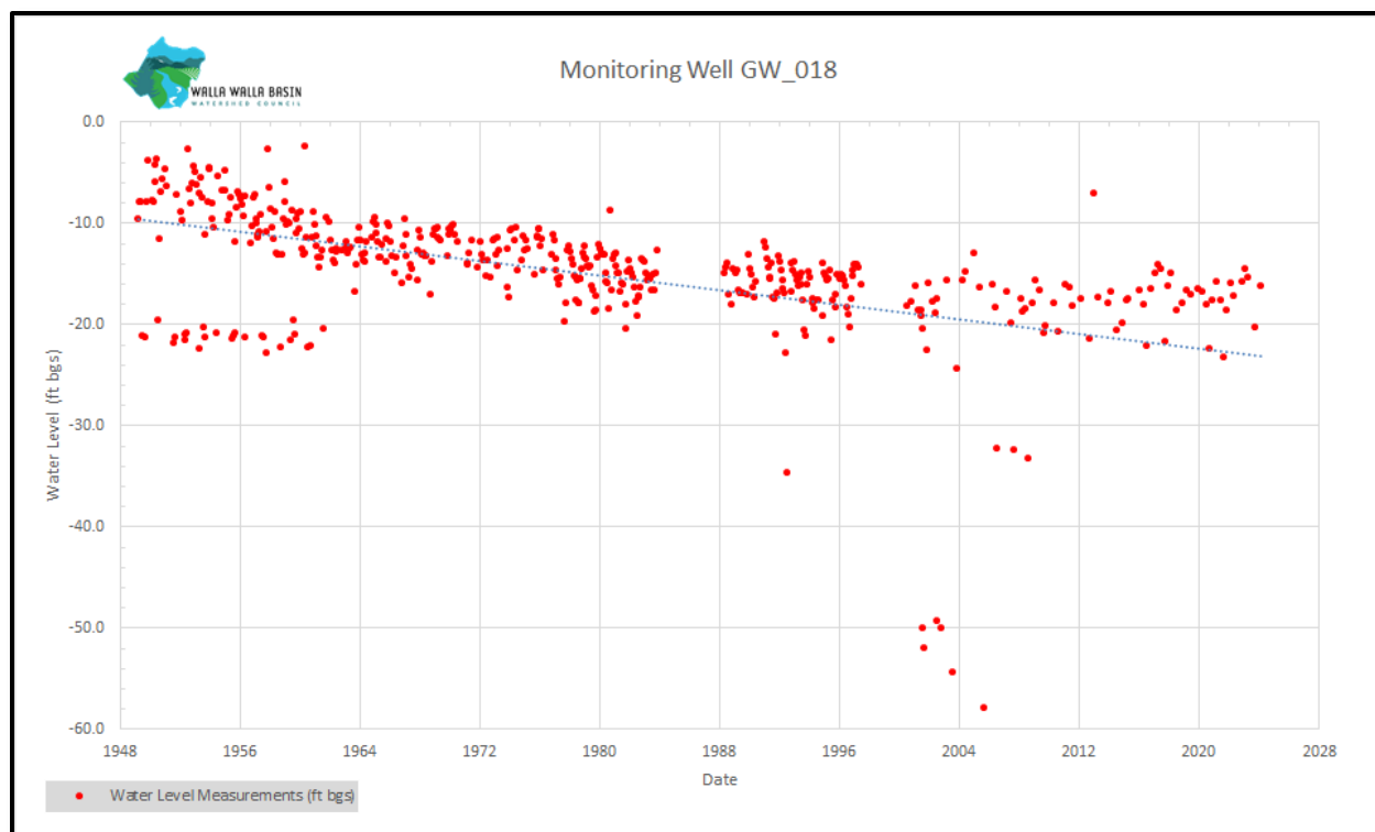
Figure 30. Manual water level measurements (red dots) and a trend line (blue dash line) for the well GW_018 located in the WWBWC's Shallow Aquifer Monitoring Network.
