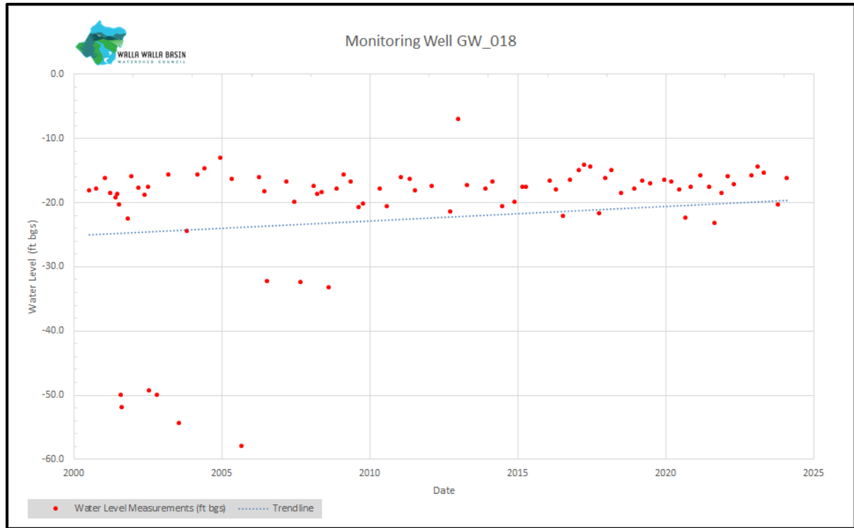
Figure 31. Manual water level measurements (red dots) and a trend line (blue dash line) since 2000 for the well GW_018 located in the WWBWC's Shallow Aquifer Monitoring Network.
