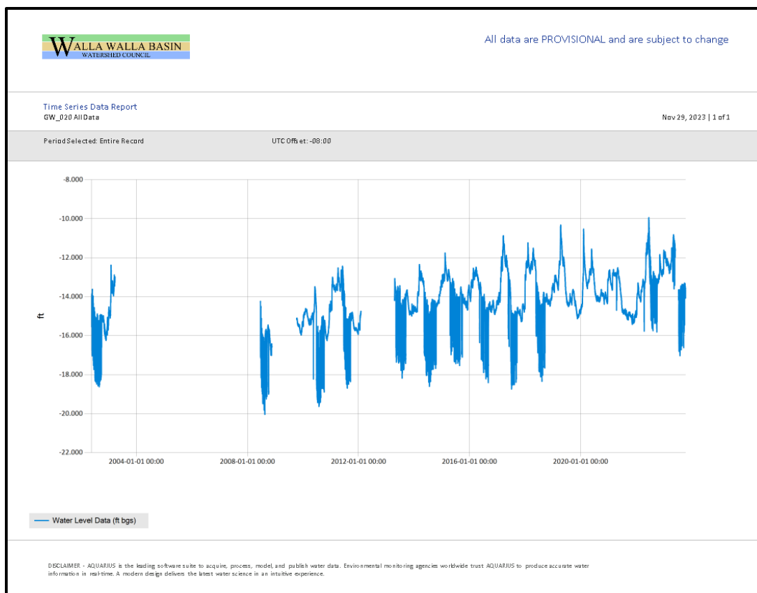
Figure 29. Pressure transducer data (blue line) in feet below ground surface for the well GW_020 located in the WWBWC's Shallow Aquifer Monitoring Network.
