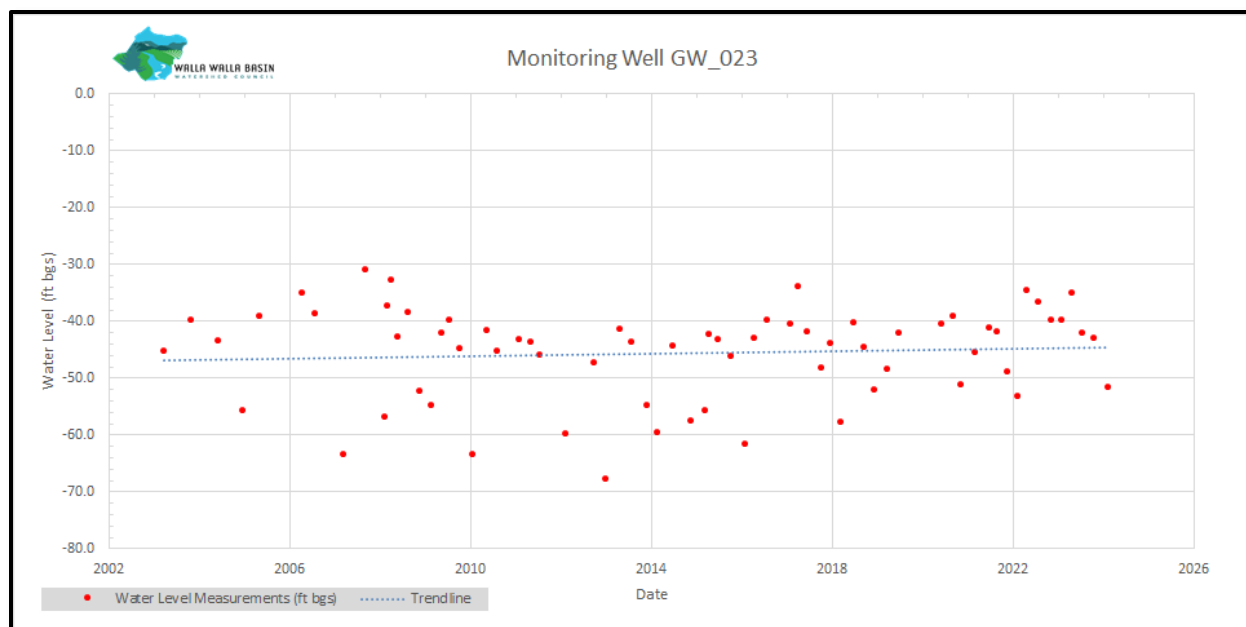
Figure 34. Manual water level measurements (red dots) and a trend line (blue dash line) since 2002 for the well GW_023 located in the WWBWC's Shallow Aquifer Monitoring Network.
