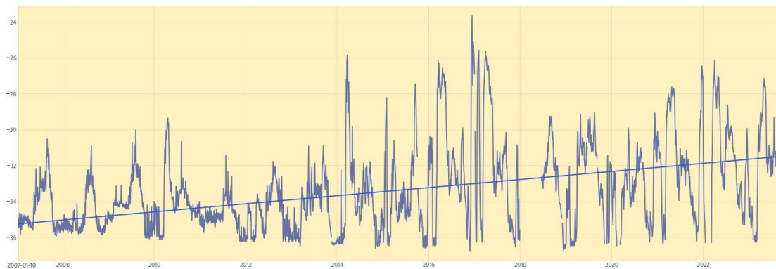
Figure 18. Pressure transducer data (blue line) in feet below ground surface and a trendline for the well GW_062 located in the WWBWC's Shallow Aquifer Monitoring Network.
