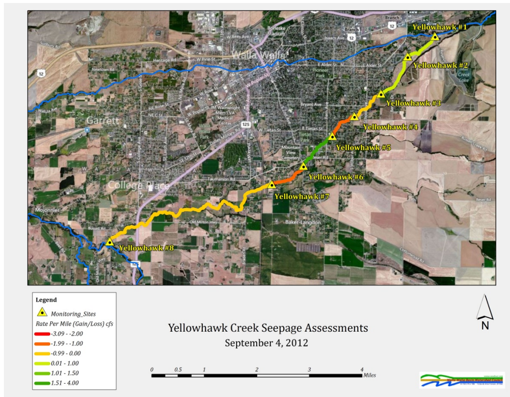
Figure 30: September 4, 2012 Yellowhawk Seepage Assessment Gaining and Losing Reaches and Rates Per Mile.
