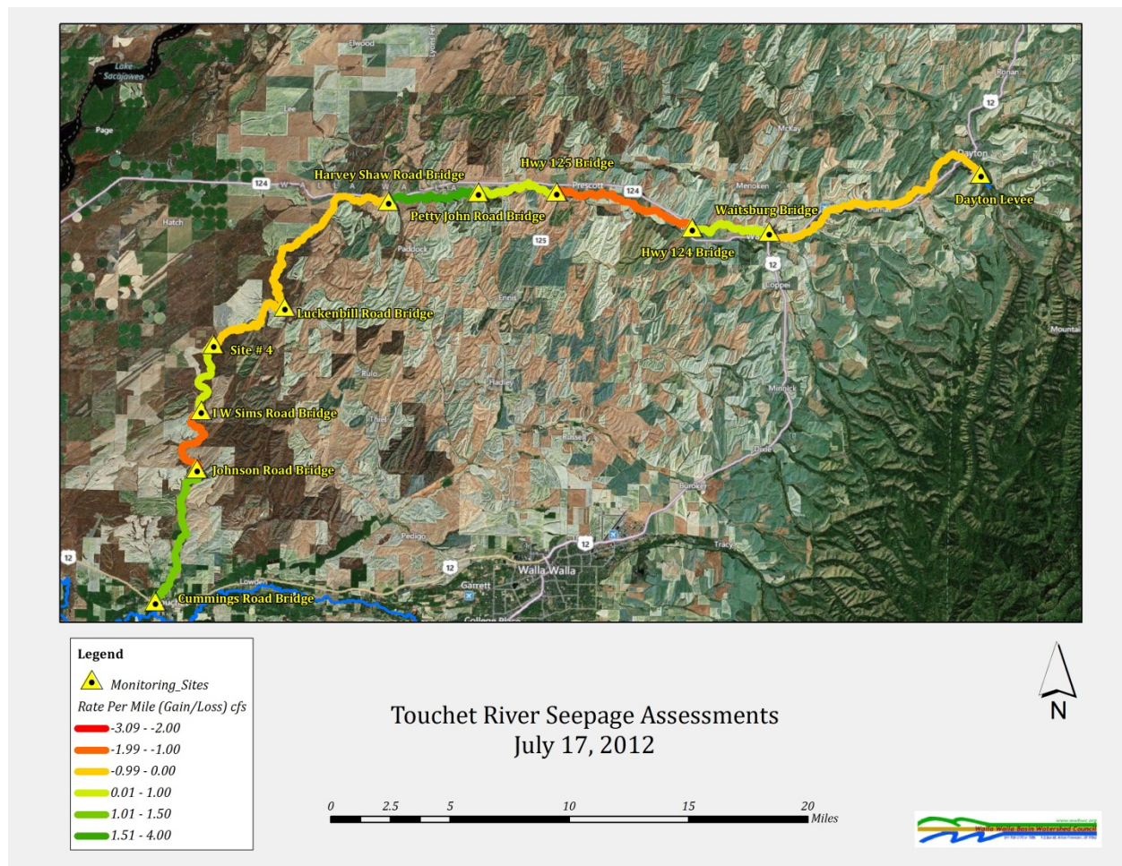
Figure 20: Touchet River Seepage Assessment July 17, 2012 Rate Per Mile (Gains and Losses) per Reach
