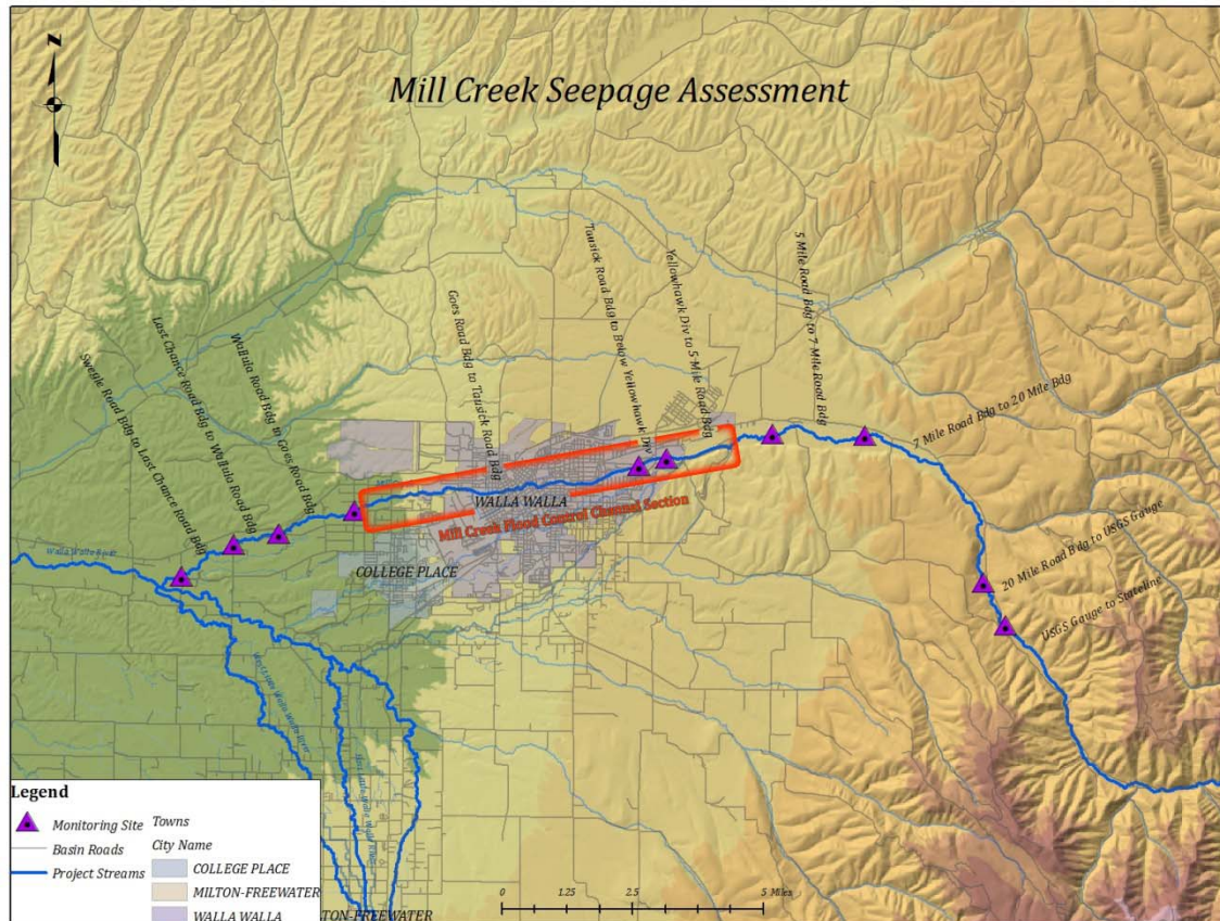
Figure 12: Mill Creek designated project reaches, 2012
