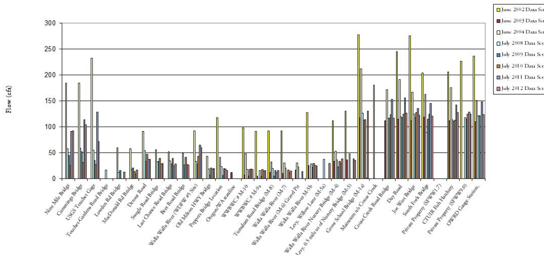
B-1: 2002-2012 June and July Longitudinal Flow Profile
