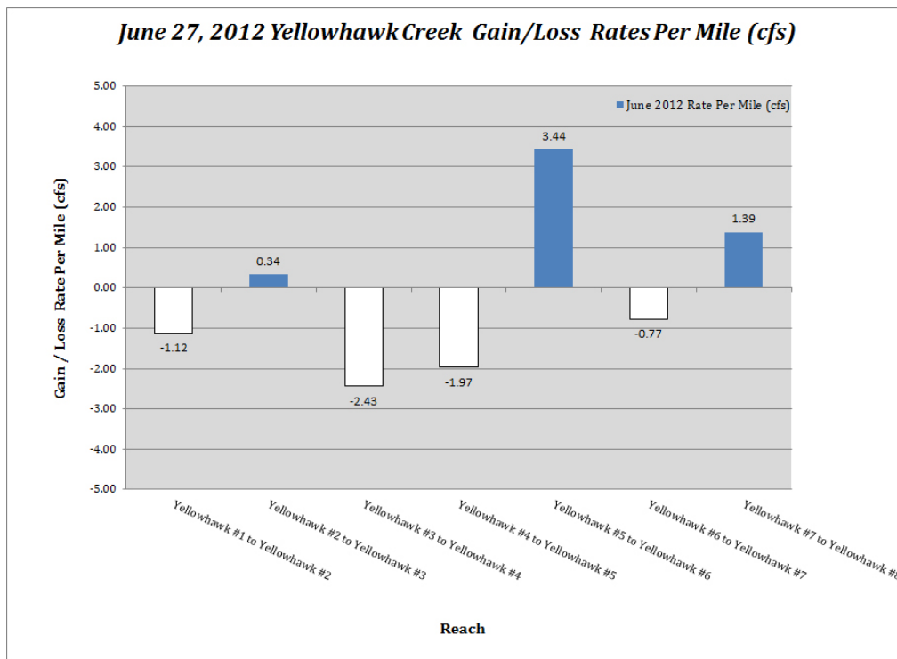
Figure 29: Yellowhawk Creek Net Channel Bed Gains/Losses (Rates per Mile) June 27, 2012
