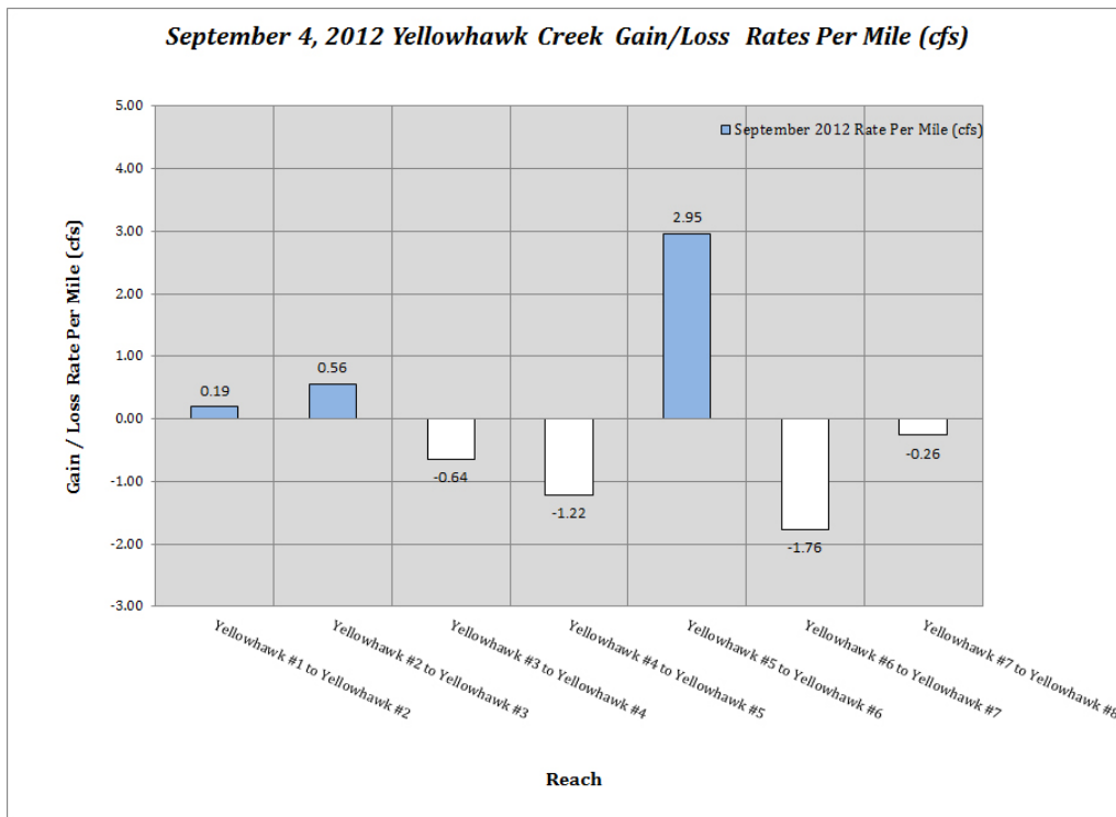
Figure 32: Net Gaining / Losing Reaches and Rate per Mile September 4, 2012
