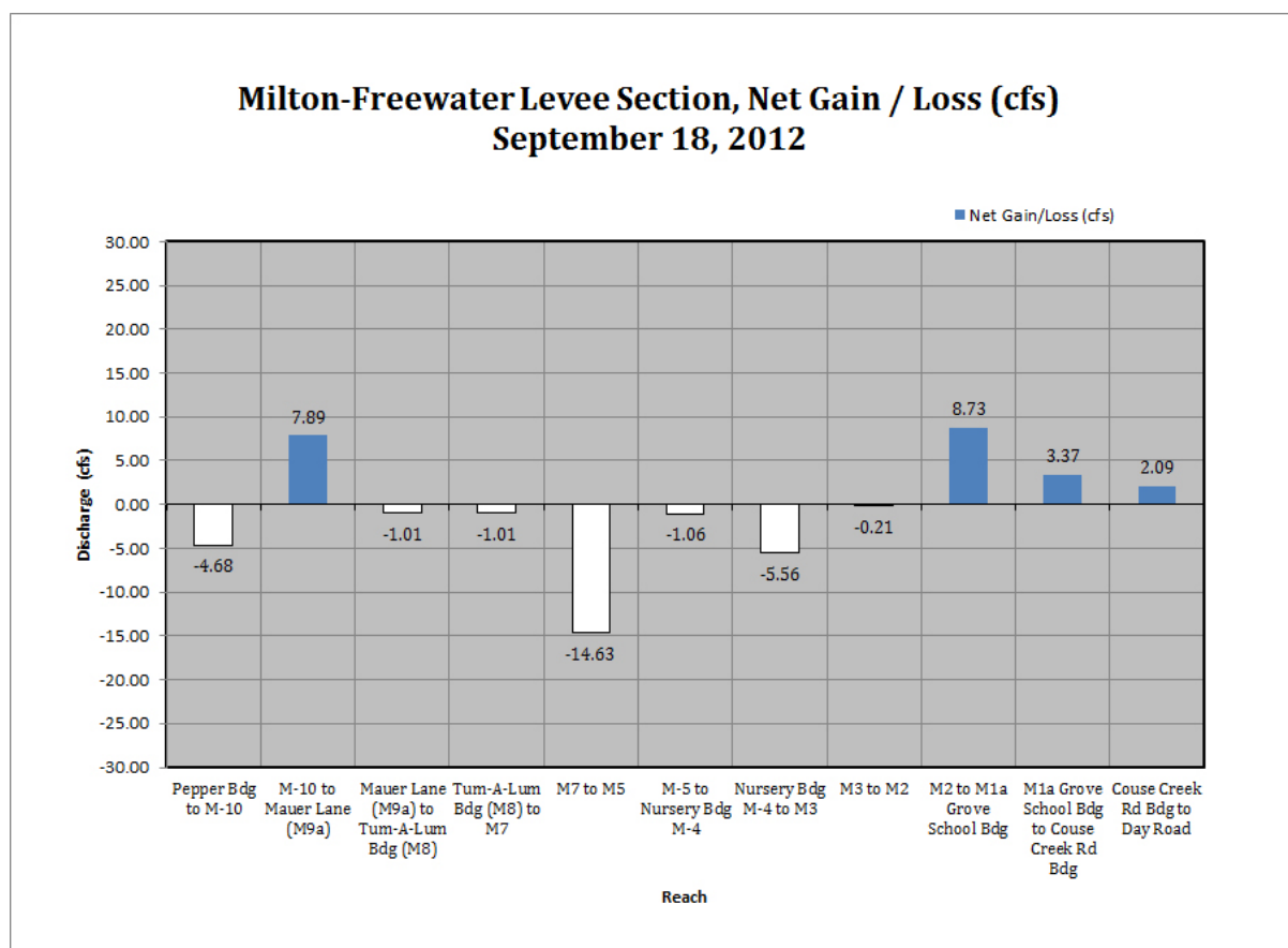
Figure 35: Milton Freewater Levee Section, Walla Walla River, September 18, 2012
