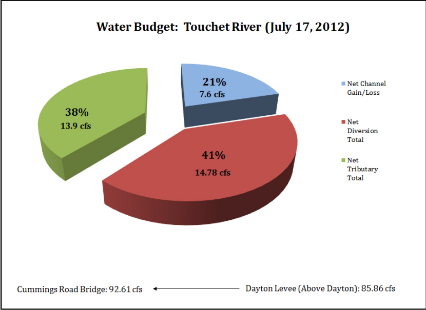
Figure 24: Water Budget July 17, 2012
