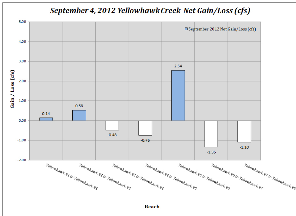
Figure 31: Yellowhawk Creek Net Channel Bed Gain/Loss September 4, 2012
