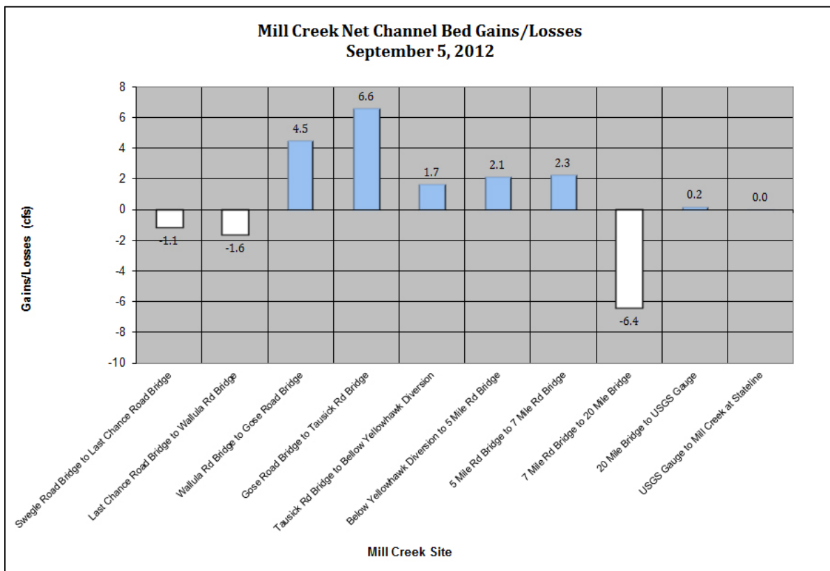
Figure 16: September 5, 2012 Net Gains and Losses Per Reach
