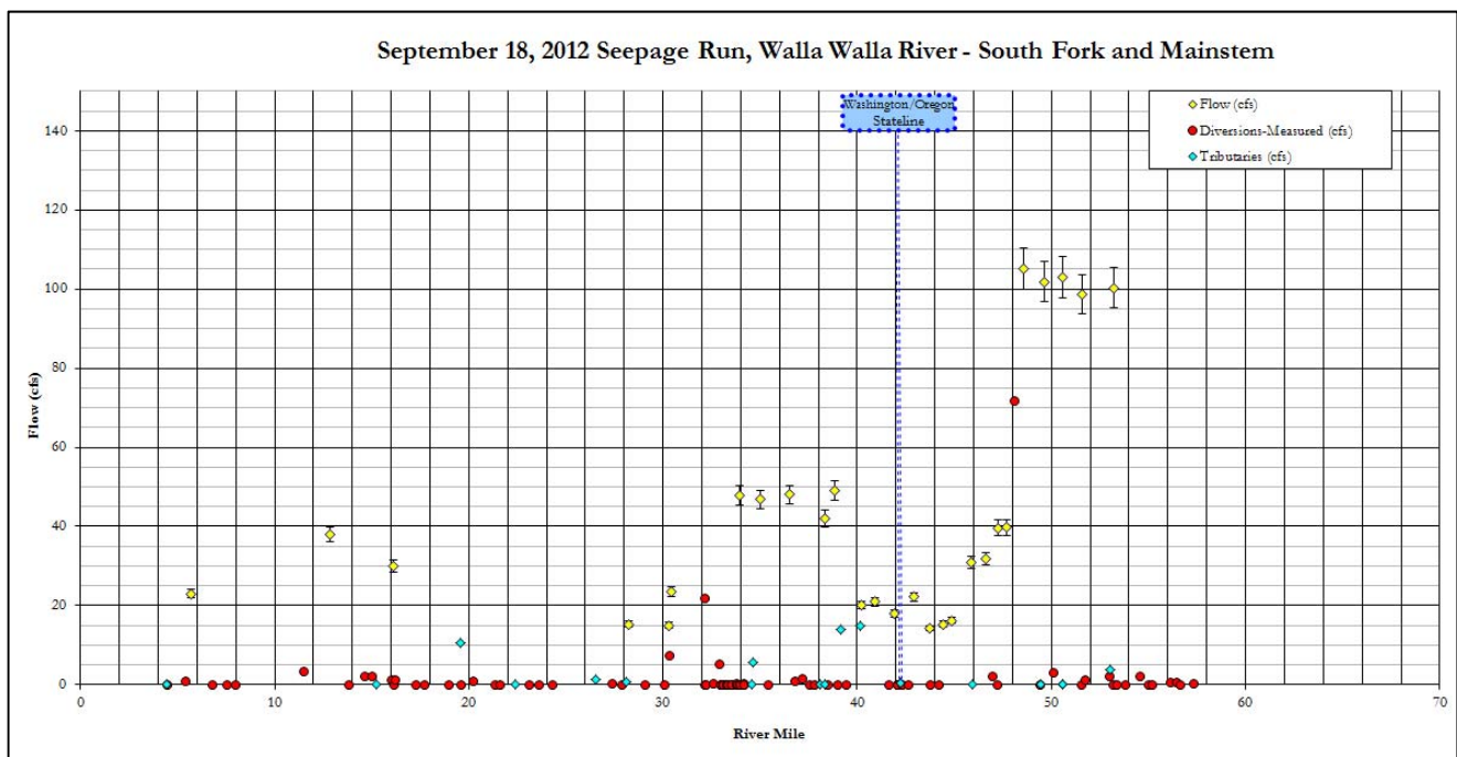
Figure 5: September 18, 2012 Walla Walla River Flow Profile
