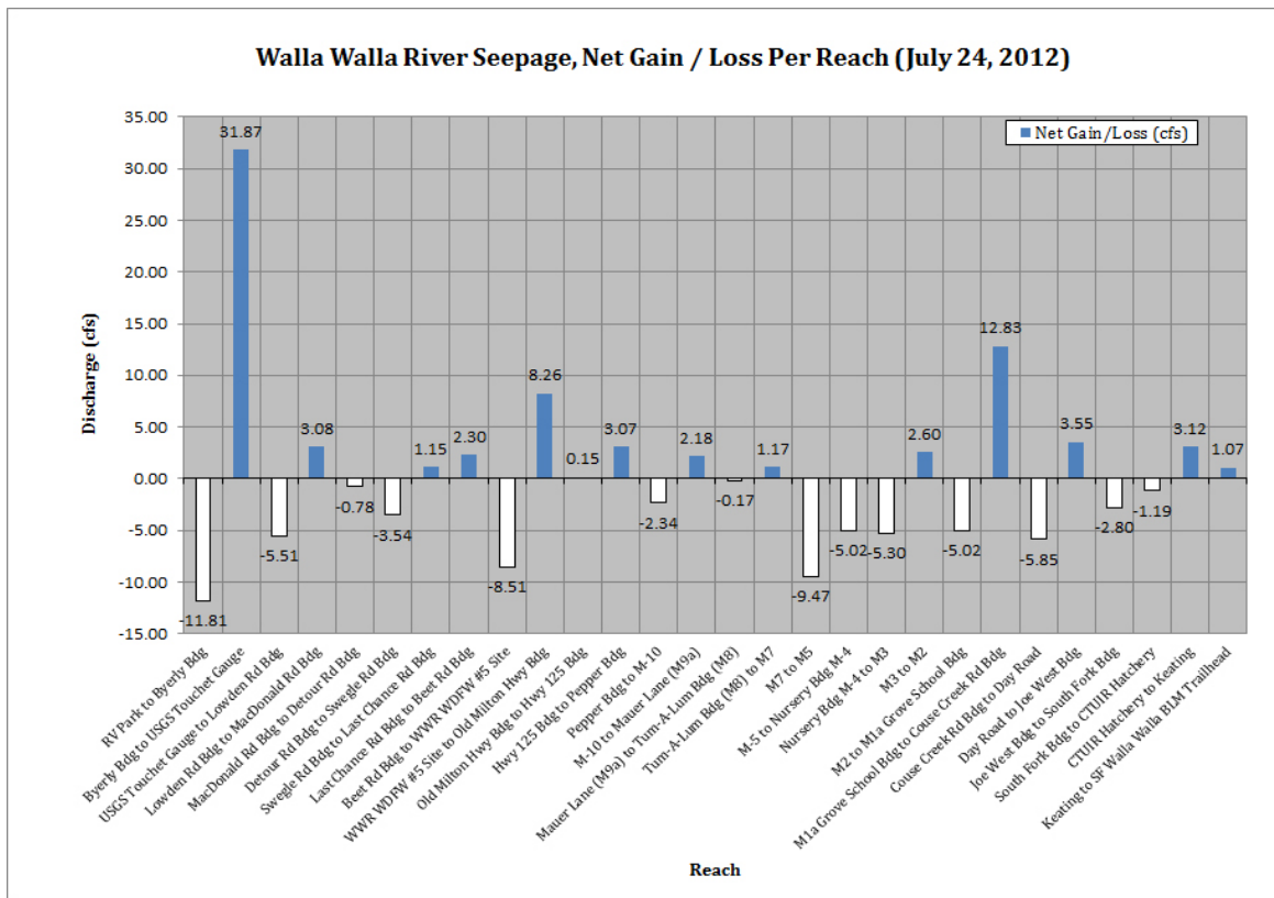
Figure 6: Walla Walla River Net Gain or Loss per Reach, July 24, 2012
