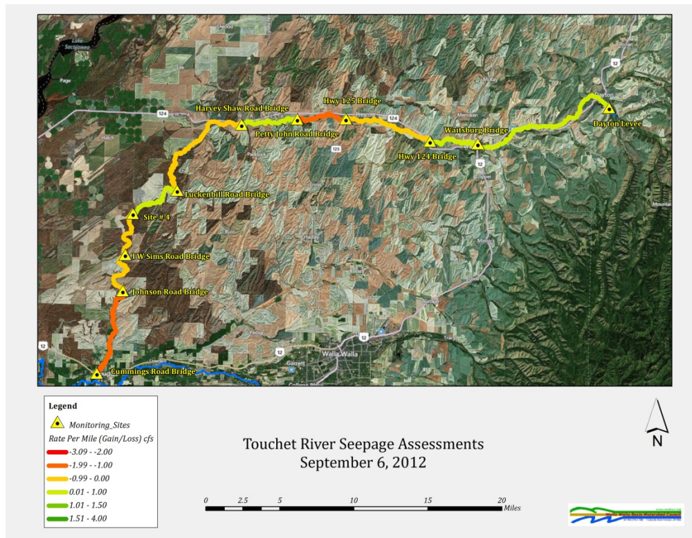
Figure 22: Touchet River Seepage Assessment September 6, 2012 Gains and Losses per Reach
