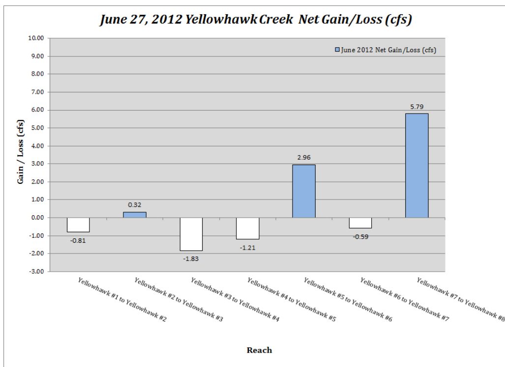
Figure 28: June 27, 2012 Yellowhawk Gains and Losses per Reach
