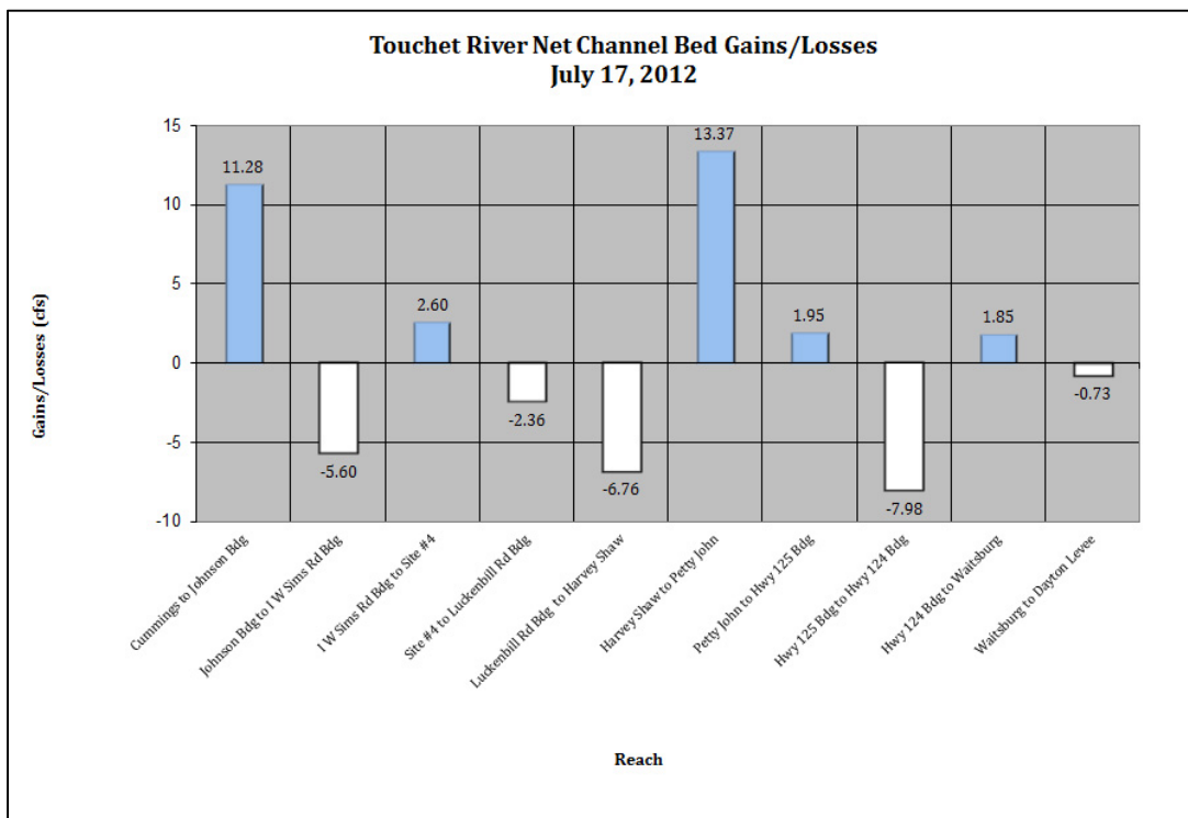
Figure 21 July 17, 2012 Net Gains and Losses per Reach
