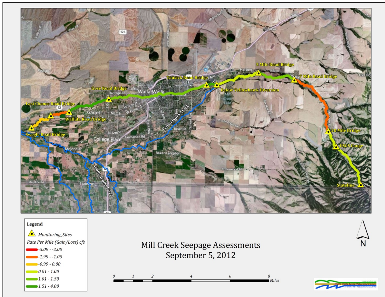
Figure 15: September 5, 2012 Mill Creek Gains / Losses per Reach
