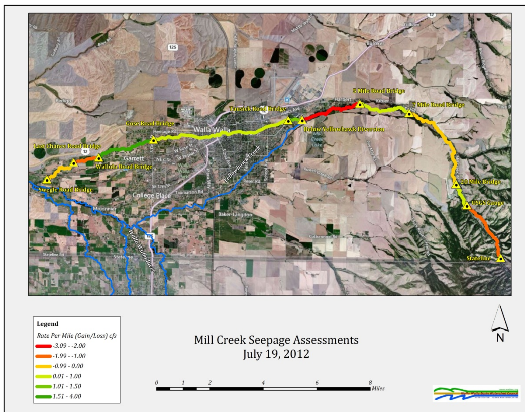
Figure 13: July 19, 2012 Mill Creek Seepage Assessment depicting the gaining and losing reaches within the assessment area
