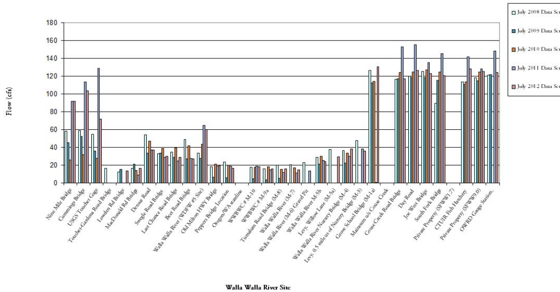
B-4: 2008-2012 July Longitudinal Flow Profile
