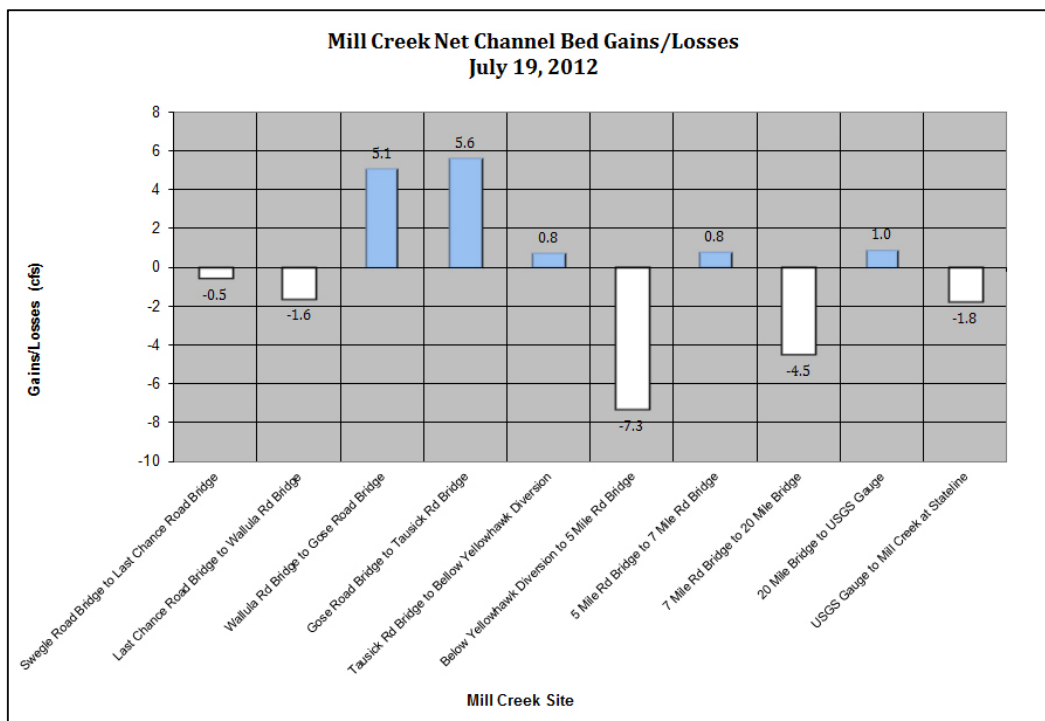
Figure 14: July 19, 2012 Seepage Assessment Net Gains and Losses per Reach
