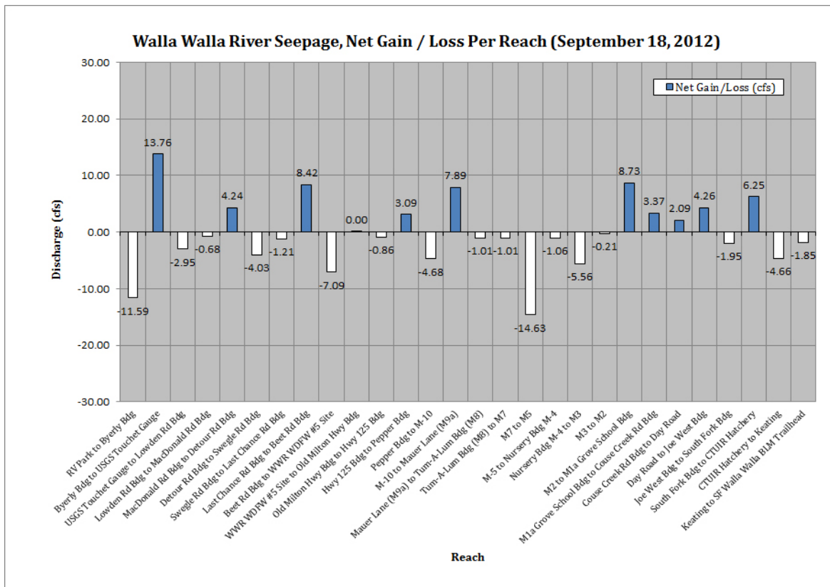
Figure 7: Walla Walla River Net Gain or Loss per Reach, September 18, 2012
