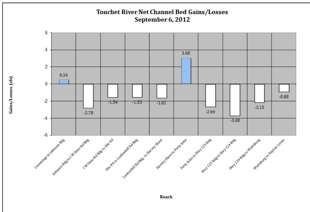
Figure 23: September 6, 2012 Net Gains and Losses per Reach
