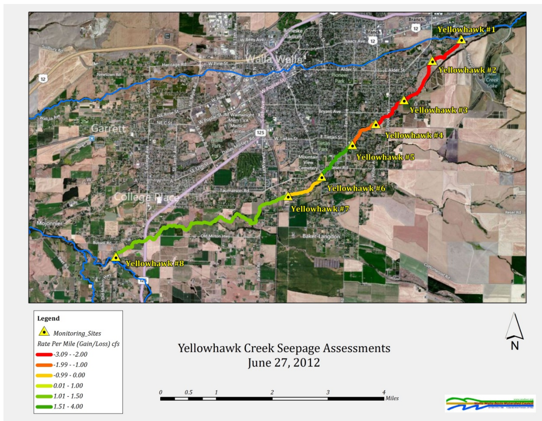
Figure 27: Net Gaining / Losing Reaches, June 27, 2012
