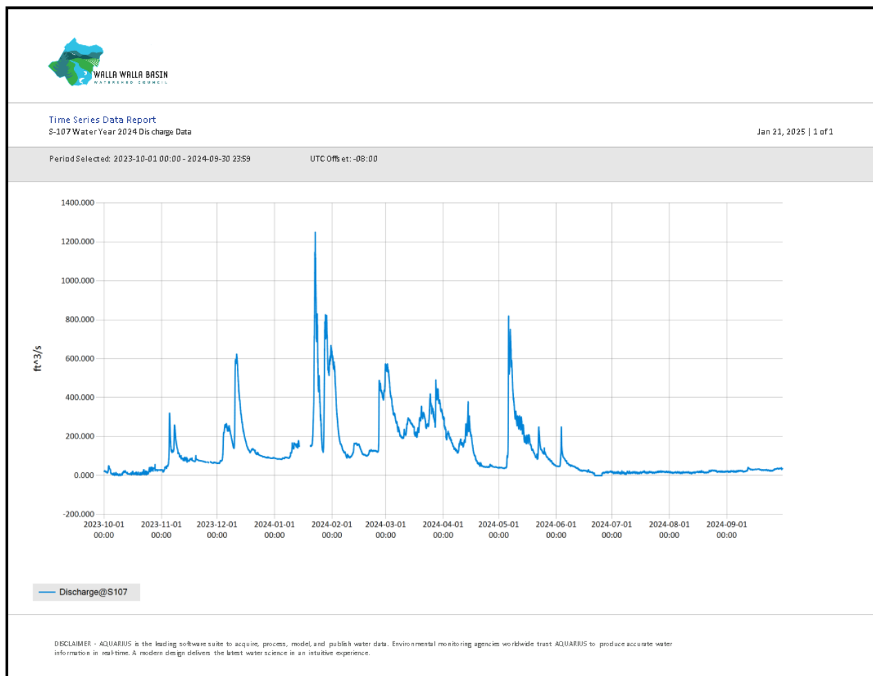
Figure 18. Walla Walla River below Tum-A-Lum Bridge (S-107) 2024 Water Year Discharge.
