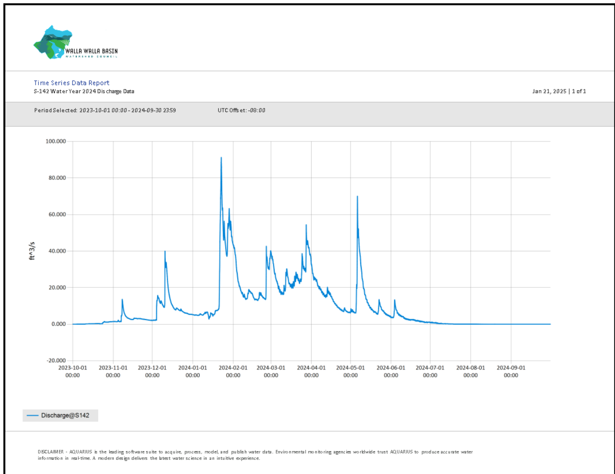
Figure 20. Couse Creek at River Mile 1.1 (S-142) 2024 Water Year Discharge.
