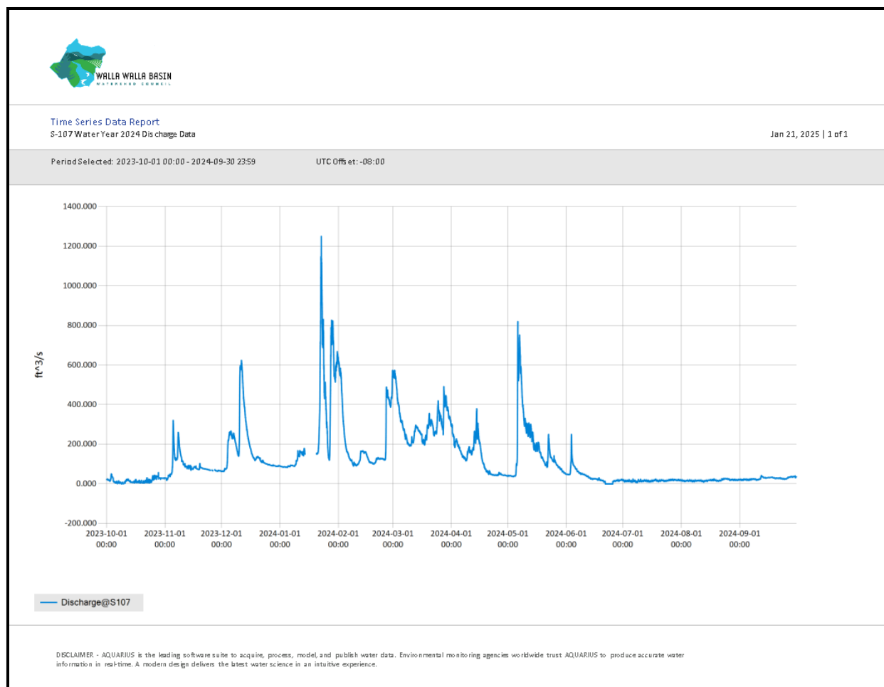
Figure 10. Walla Walla River below Tum-A-Lum Bridge (S-107) flow data computed by processing stage data through the rating curve shown in Figure 8.
