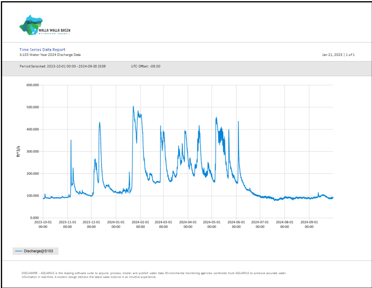
Figure 12. South Fork Walla Walla River near Confluence (S-103) 2024 Water Year Discharge.
