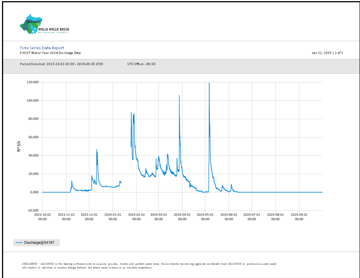
Figure 22. Pine Creek at Schubert Road (S-416T) 2024 Water Year Discharge.
